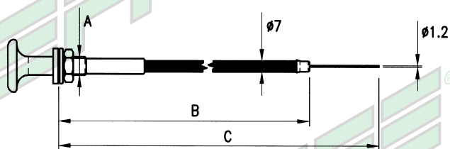
M25 - COMANDO STOP MOTORE M25 - STOP ENGINE CONTROL M25 - MOTORABSTELLZUG
